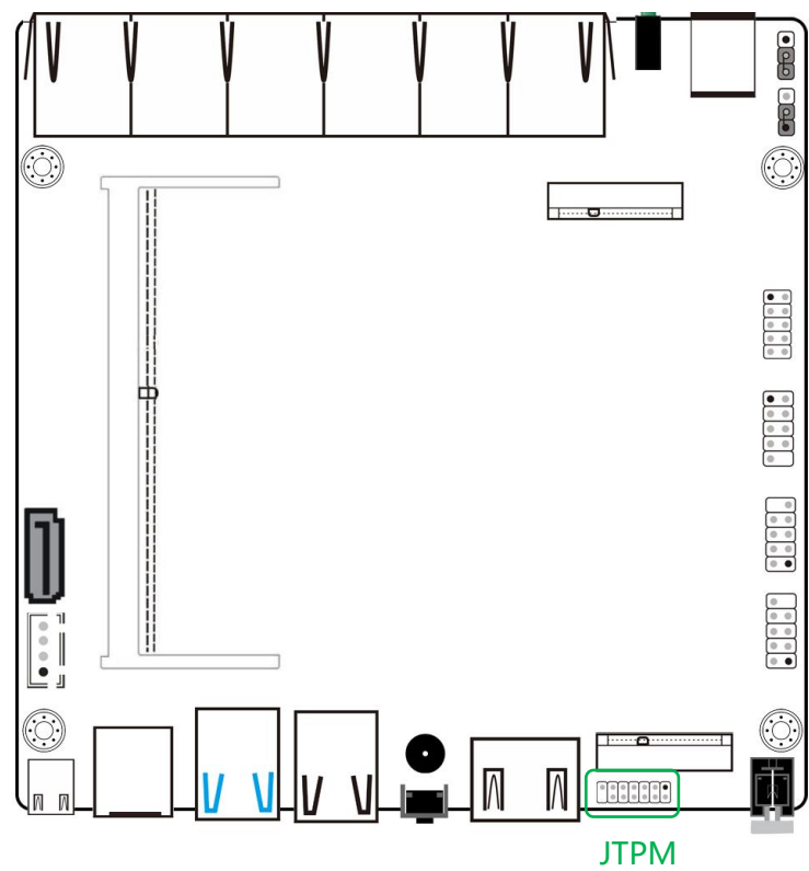
JTPM (2×7 pin 间距 2.00mm)
